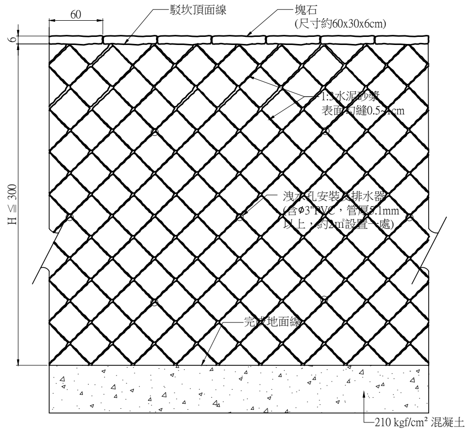
漿砌整形塊石排列示意圖 A1 (1:20) A3 (1:40) Unit:cm
