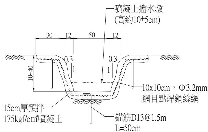
噴漿溝詳圖 NTS Unit:cm
