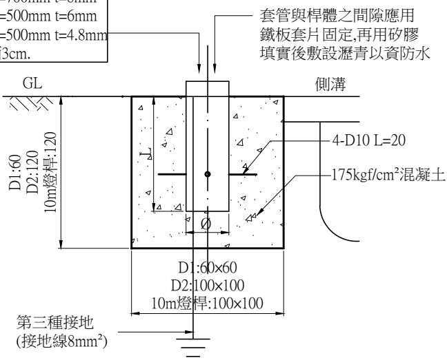
套管式燈桿基礎 TYPE(T) NTS Unit:cm
