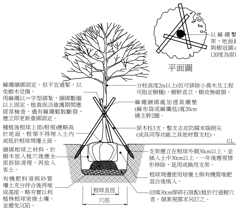
喬木栽植立支架示意圖(三柱式) NTS Unit:cm
