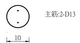
Ø10cm 仿松欄杆配筋 A1 (1:5) A3 (1:10) Unit:cm
